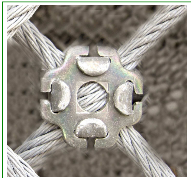
Pannelli in fune a nodi borchiati mod. INCOPAN HCP
